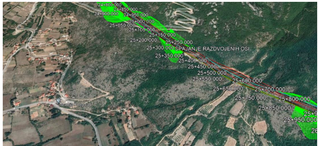
Figure 3-50: Intersection of local road with motorway in Seocka Draga (source: Google Earth)
