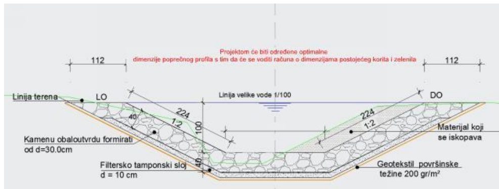
Figure 3-16: Typical cross section of training structure
