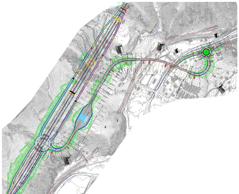
Figure 3-10: Beginning of the subsection Ovcari - Prenj Tunnel with Ovcari interchange
