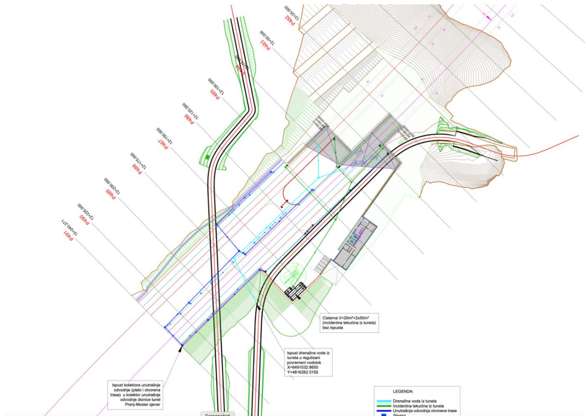
Figure 3-38: Purification system solution for drainage water from the Prenj tunnel on the south side
