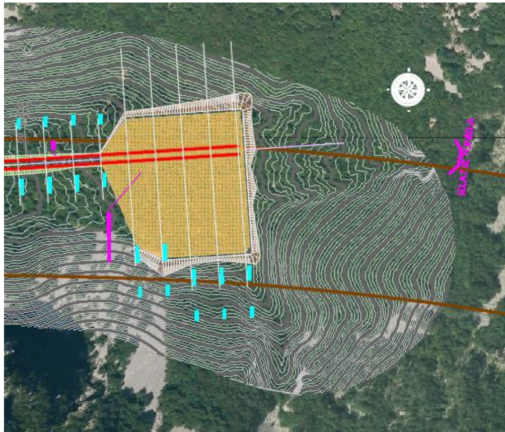
Figure 3-33: Design situation of the section SR6, operational plateau 3
