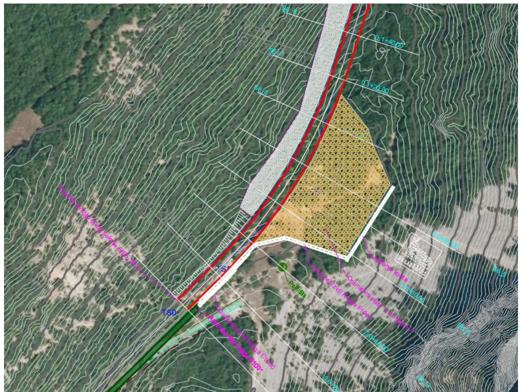
Figure 3-31: Design situation of the section SR6, operational plateau 1
