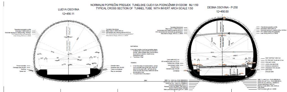
Figure 3-21: Normal cross section of the Prenj tunnel
