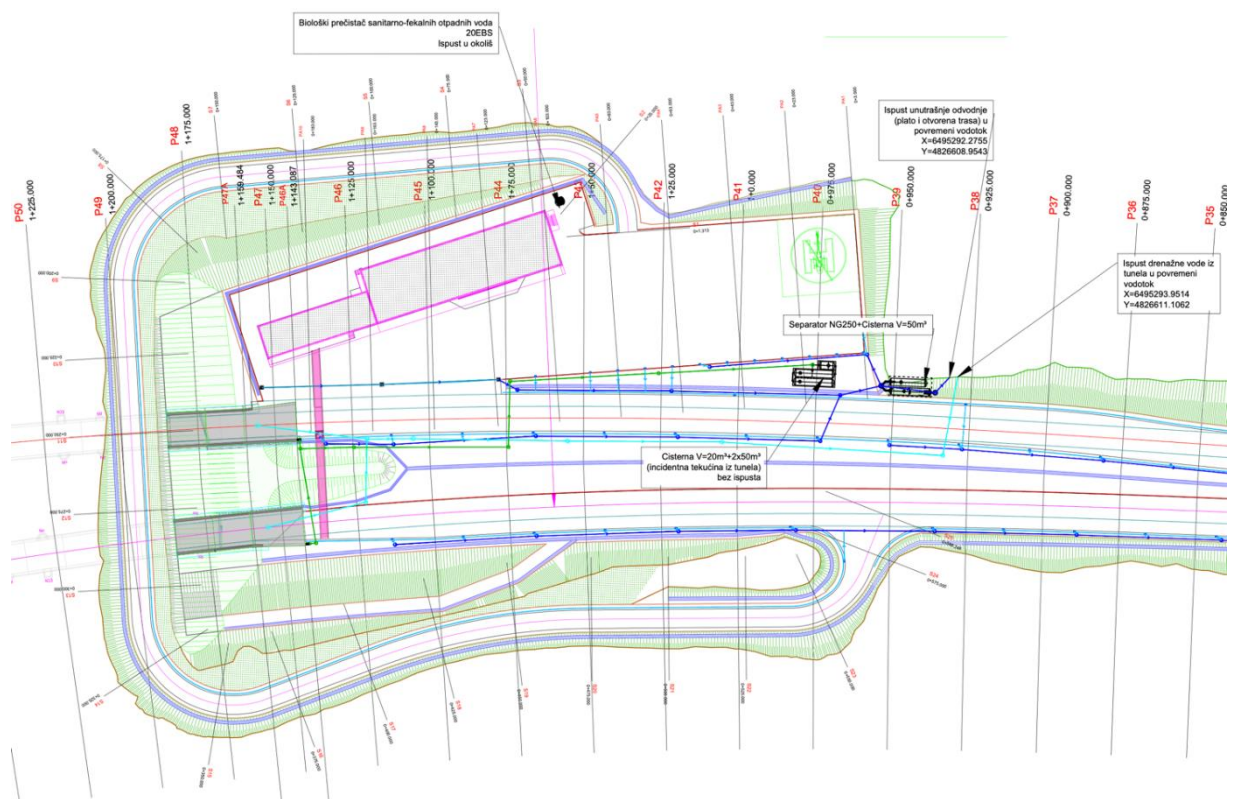
Figure 3-37: Purification system solution for drainage water from the Prenj tunnel on the north side
