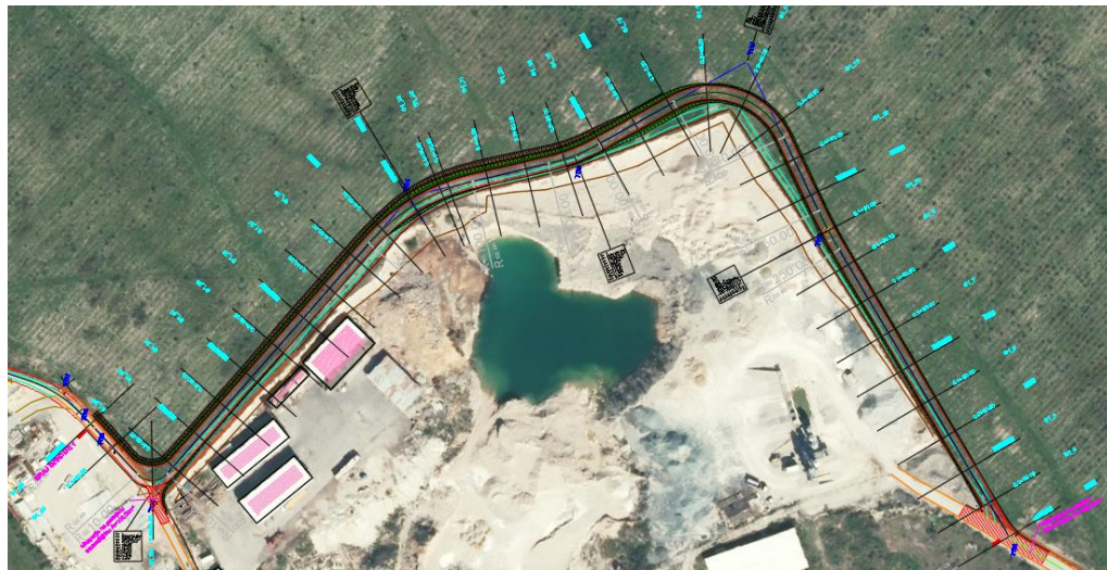
Figure 3-29: Design situation of the section SR1
