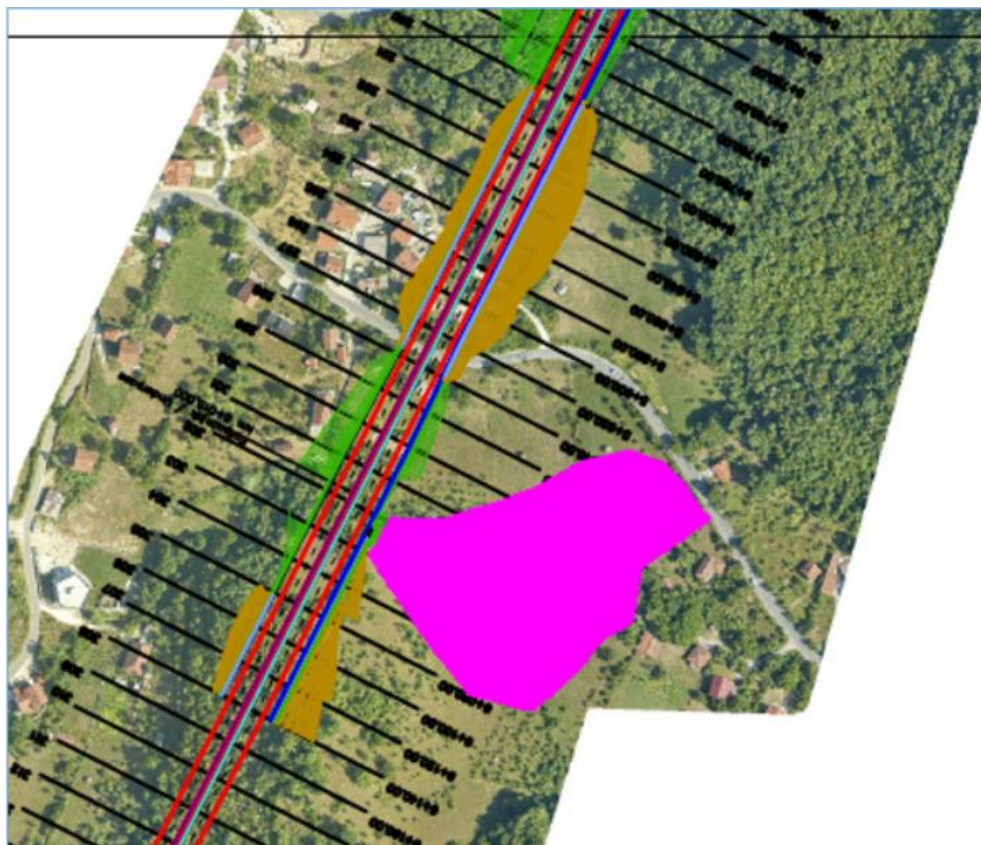
Figure 3-46: Landscaping area between regional road diversion and motorway
