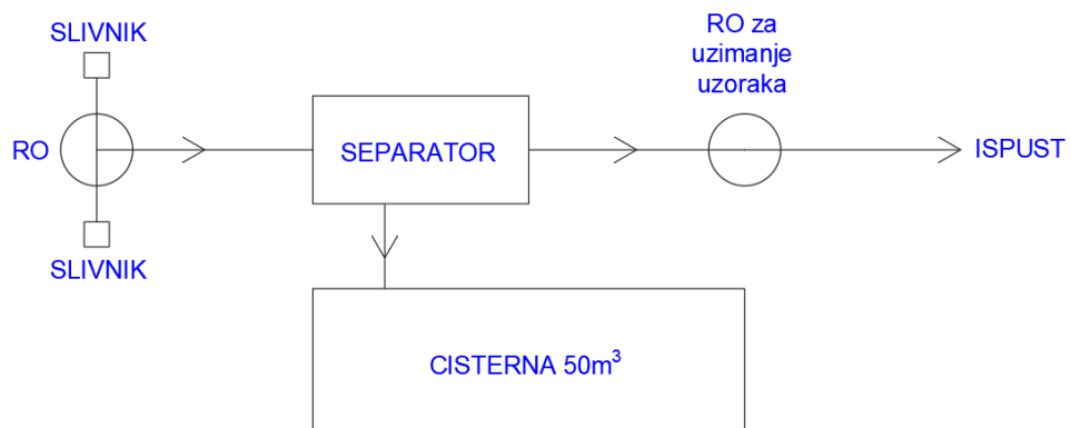
Figure 3-40: Hydraulic scheme of purification process in high risk zones of subsection tunnel Prenj-Mostar North
