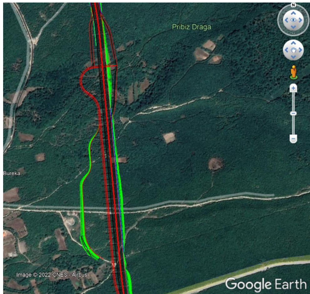
Figure 3-23: Design situation of the rest area (source: Google Earth)
