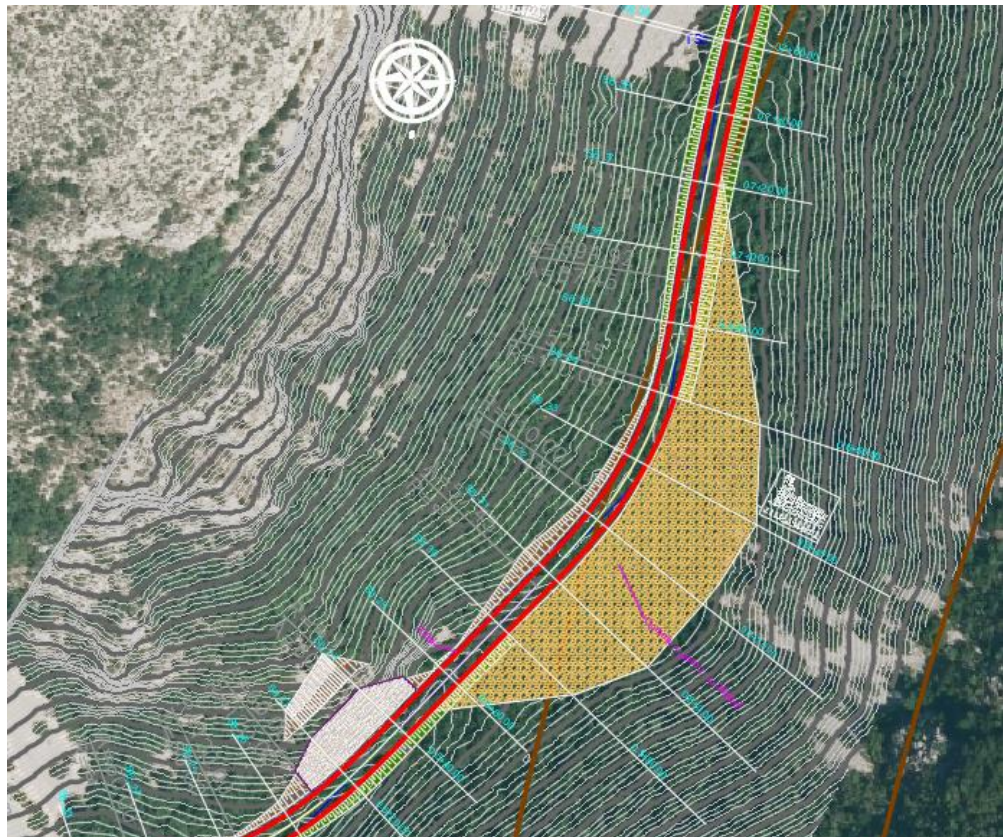
Figure 3-32: Design situation of the section SR6, operational plateau 2
