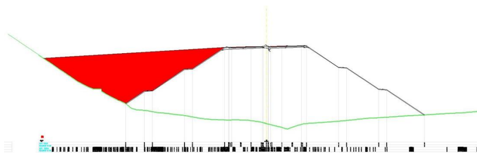
Figure 3-45: Embankment profile on Section 3
