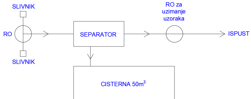
Figure 3-34: Hydraulic purification scheme in case of discharge upstream of the captured springs on the subsection Ovcari–entrance to the Prenj tunnel
