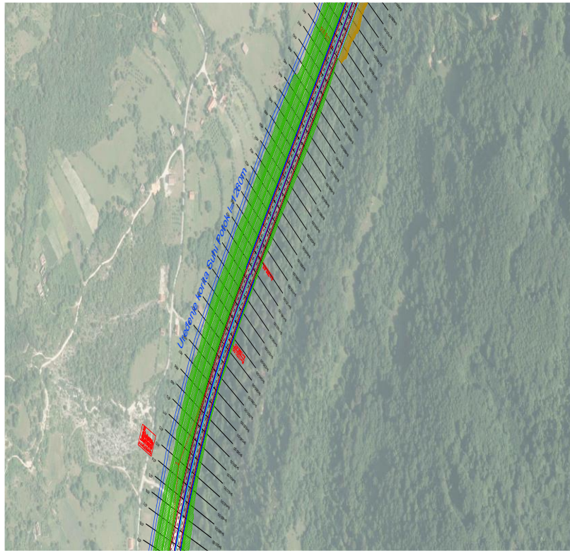
Figure 3-20: Training of the Suhi potok stream (L=1,280 m)
