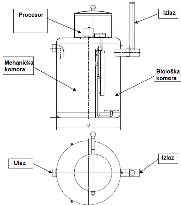
Figure 3-36: Schematic representation of the SBR device planned for the subsection Ovcari-entrance to the Prenj tunnel
