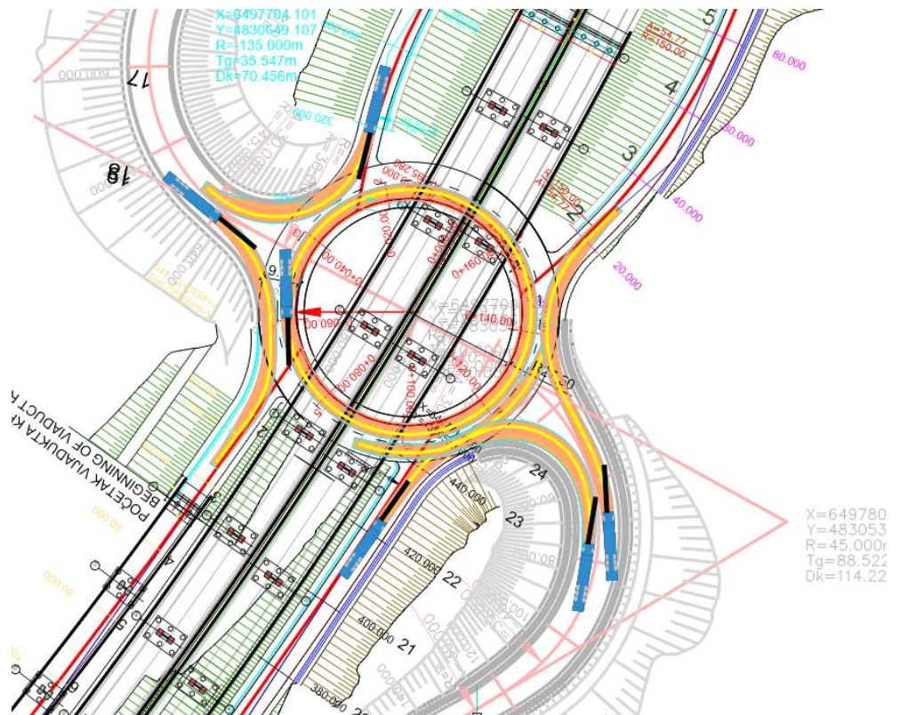
Figure 3-18: Design of the Konjic South interchange
