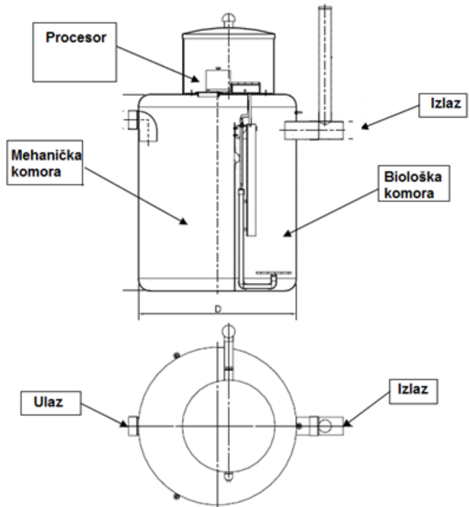
Figure 3-41: Schematic representation of the SBR device for tunnel Prenj-Mostar North subsection
