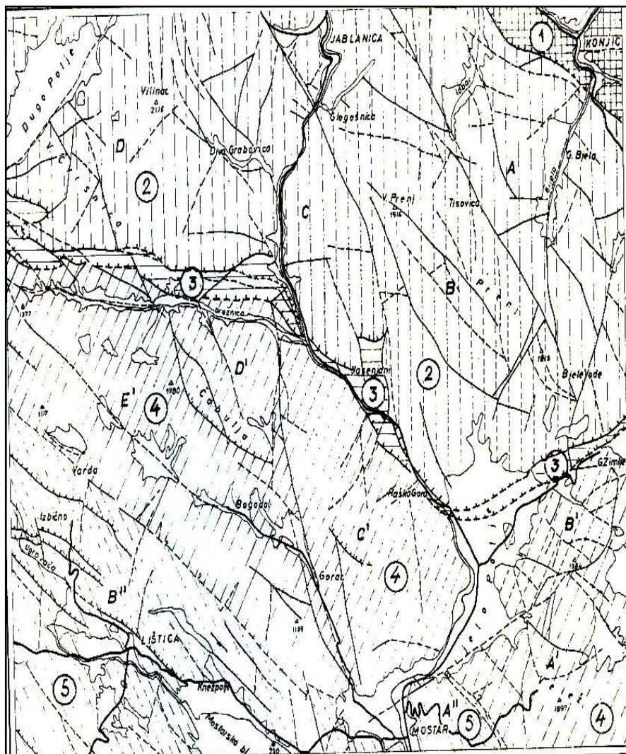
Figure 7-11: Generalized tectonic map of the Sheet Mostar 3
